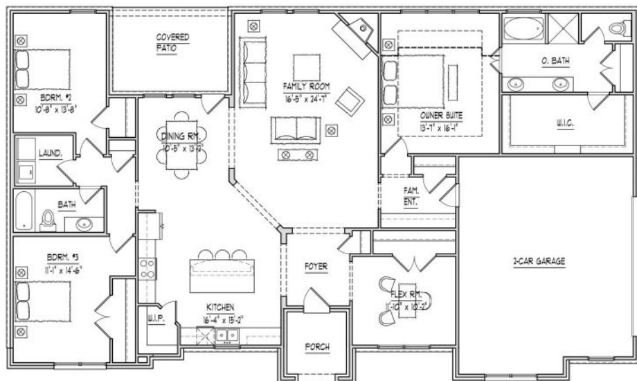
FIRST FLOOR PLAN ELEVATION C
